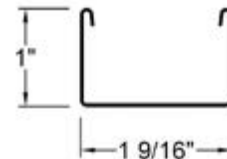
Optional Commercial Headrail
