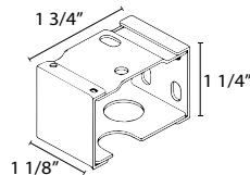
Optional Commercial Headrail 50-04-037-XXX
