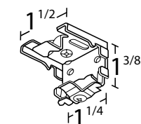
Echelon/Integra Bracket 59-08-135 7/8" Spacer 59-07-890 1/2" Spacer 59-07-230 Hold Down 15-2009
